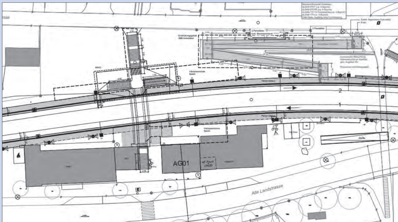
Abb. 4: Plan Rampe
